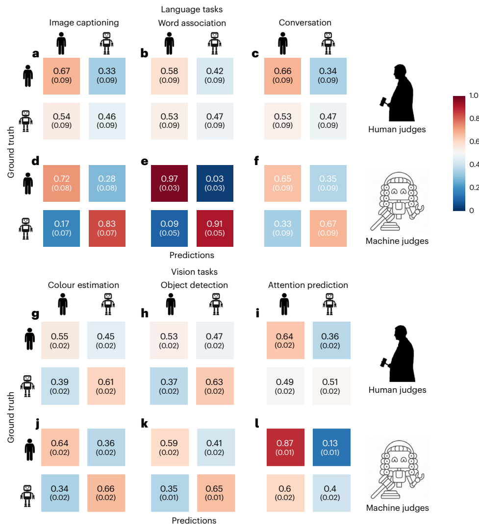
Fig. 4 | Results of the Turing-like test for each task. a–l, Turing-like test results for human judges (a–c) and machine judges (d–f) in language tasks and human judges (g–i) and machine judges (j–l) in vision tasks. Each column shows the results for a different task: image captioning (a,d), word association (b,e), conversation (c,f), colour estimation (g,j), object detection (h,k) and attention prediction (i,l). For each task, the confusion matrices report the proportion of times when the trial was labelled ‘human’ (first column) or ‘machine’ (second
