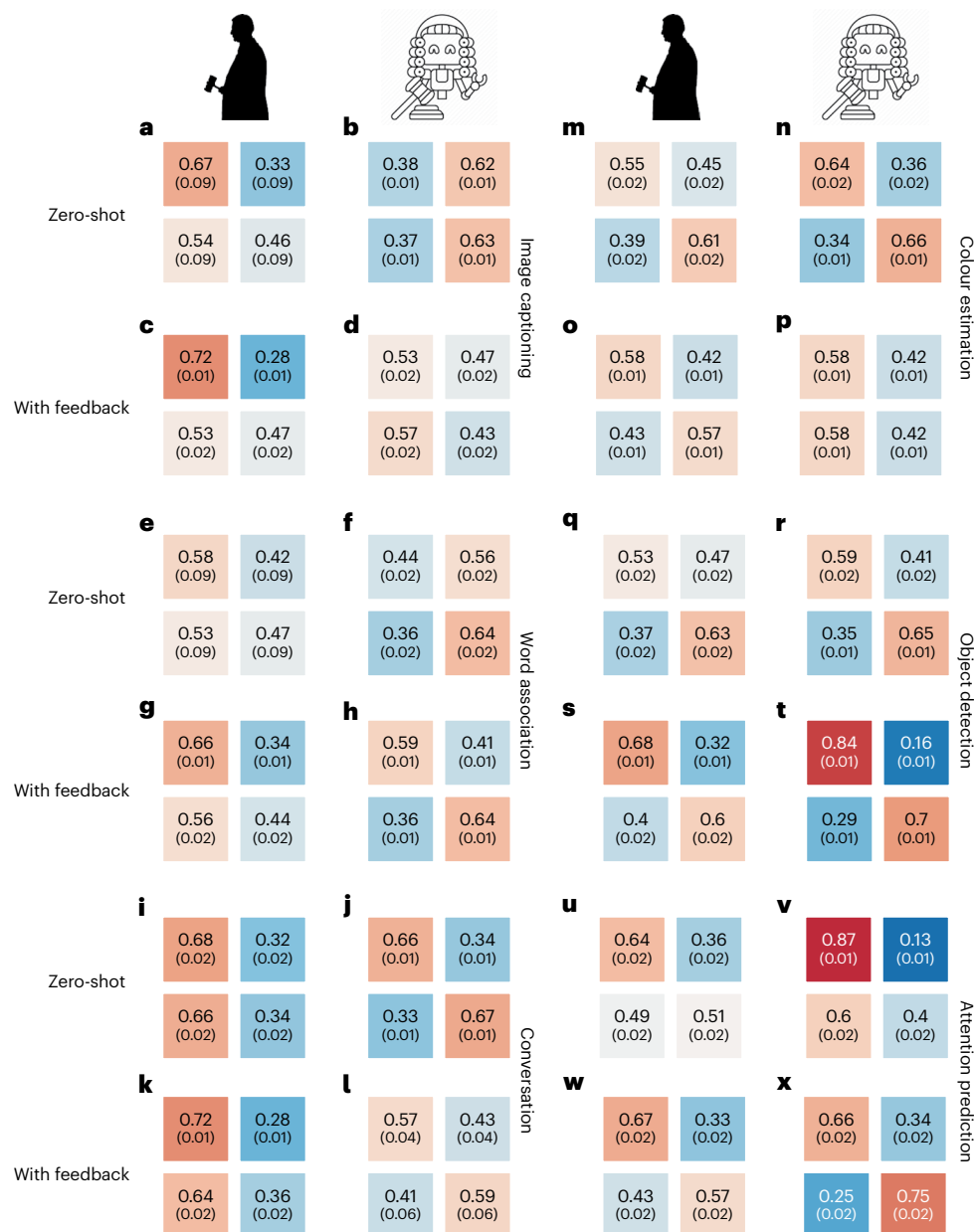
Fig. 7 | Comparison between human and machine judges in zero-shot settings or trained with feedback. a–x. Following the same format as in Fig. 4, the matrices show Turing-like test results for human judges in zero-shot settings (a, e, i, m, q, u) or trained with feedback (c, g, k, o, s, w) across all six tasks and Turing-like test results for machine judges in zero-shot settings (b, f, j, n, r, v) or
