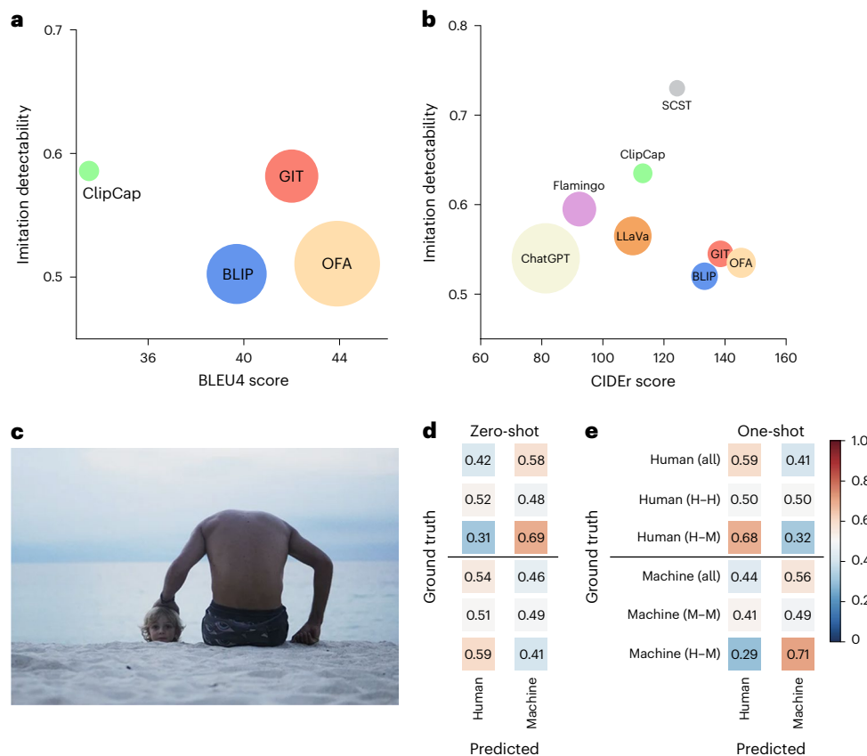
Fig. 8 | Lack of correlation between imitation detectability and standard performance metrics in the image captioning task, and Turing results in the conversation task with AI judges. a, b , Four state-of-the-art image captioning models, GIT 1 (red), OFA 2 (yellow), BLIP 3 (blue) and ClipCap 4 (green), are evaluated in terms of their imitation detectability (y axis) as a function of their BLEU score 18 ( a ) and their CIDEr score 2 ( b ). We also added four more image captioning models, OpenFlamingo-4B 52 (light purple), ChatGPT-4o-latest 12 (light yellow), SCST 53 (grey) and LLaVA-v1.6-Mistral-7B 54 (orange), for the CIDEr score ( b ). The BLEU score and the CIDEr score are standard evaluation metrics commonly used in image captioning tasks to assess the quality of the generated captions given an image on the basis of n -gram overlaps. The higher the values, the better. The radius of each circle is proportional to the AI model size in terms of the number of trainable network parameters. c , Image eliciting correct answers that do not necessarily imitate humans. In response to the query “What do you see in this image?” GPT4 answered, “In this image, a man is sitting on a sandy beach with his back to the camera, facing the ocean. Next to him, a child’s head is visible, appearing to be buried in the sand up to their neck. The man has one arm extended, resting his hand gently on the child’s head. The scene is serene
