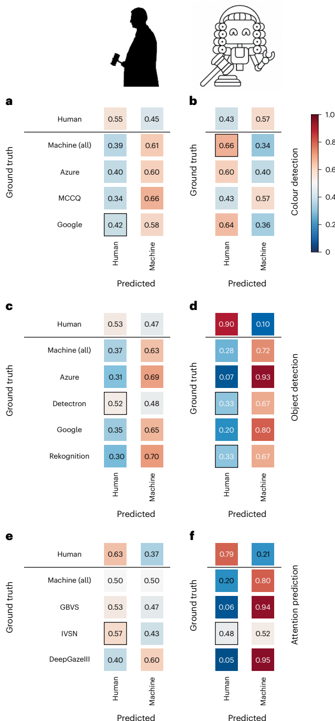
Fig. 6 | Full results of the Turing-like test for each vision task. a–f, Turing-like test results for human judges ( a, c, e ) and AI judges ( b, d, f ) in the three vision tasks: colour detection ( a, b ), object detection ( c, d ) and attention prediction ( e, f ). The full confusion matrices follow the same conventions as Fig. 4. The colour bar in b applies to all panels. The boxes with black frames denote the best algorithm in terms of its ability to pass as human—that is, highest p(H|M) .
